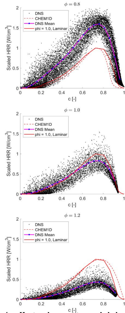
Figure 4: Heat release rate, scaled by limits of corresponding 1D unstrained flames, with respect to the progress variable. Significant deviation from 1D flame behaviour seen for rich mixture.
