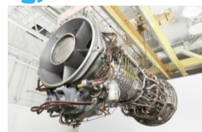
©LM2500+G4, General Electric
